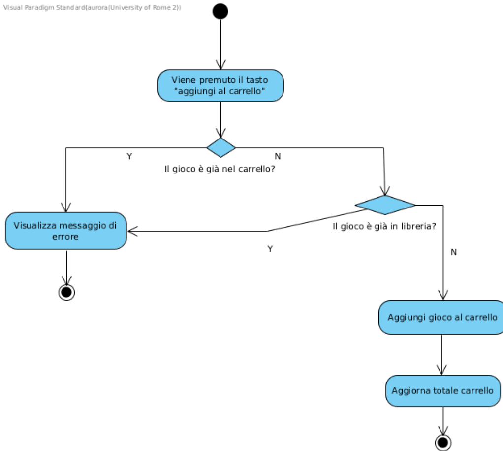
Figura 12: Activity Diagram - Gestione carrello
