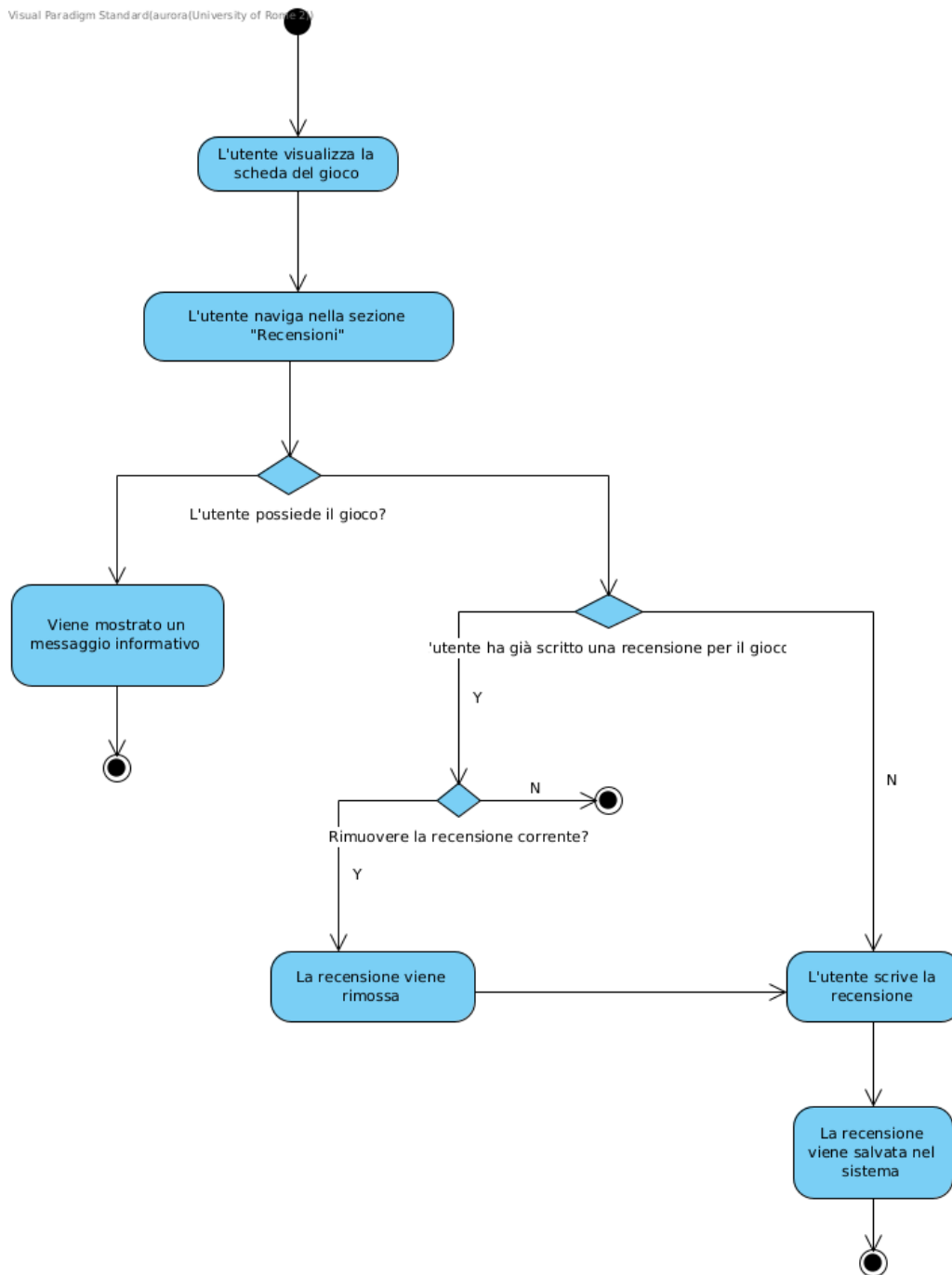
Figura 13: Activity Diagram - Recensisce
