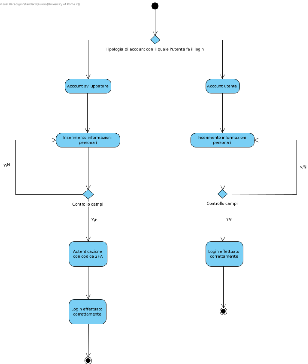
Figura 6: Activity Diagram - Login
