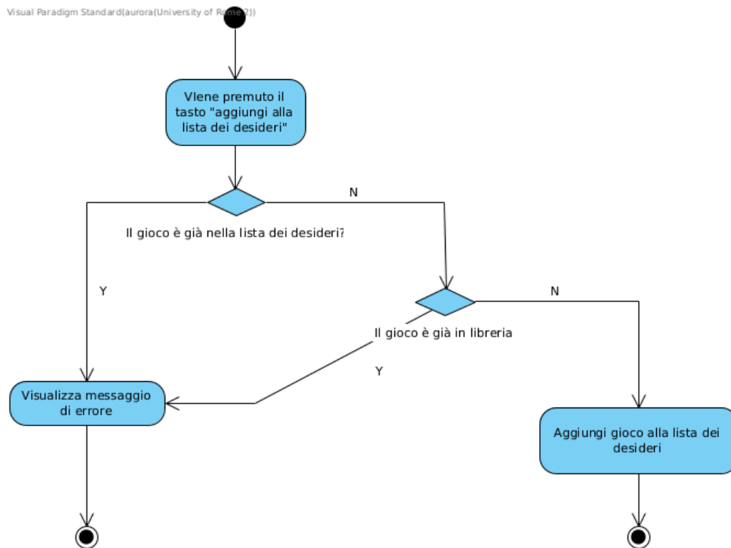
Figura 11: Activity Diagram - Gestione lista desideri
