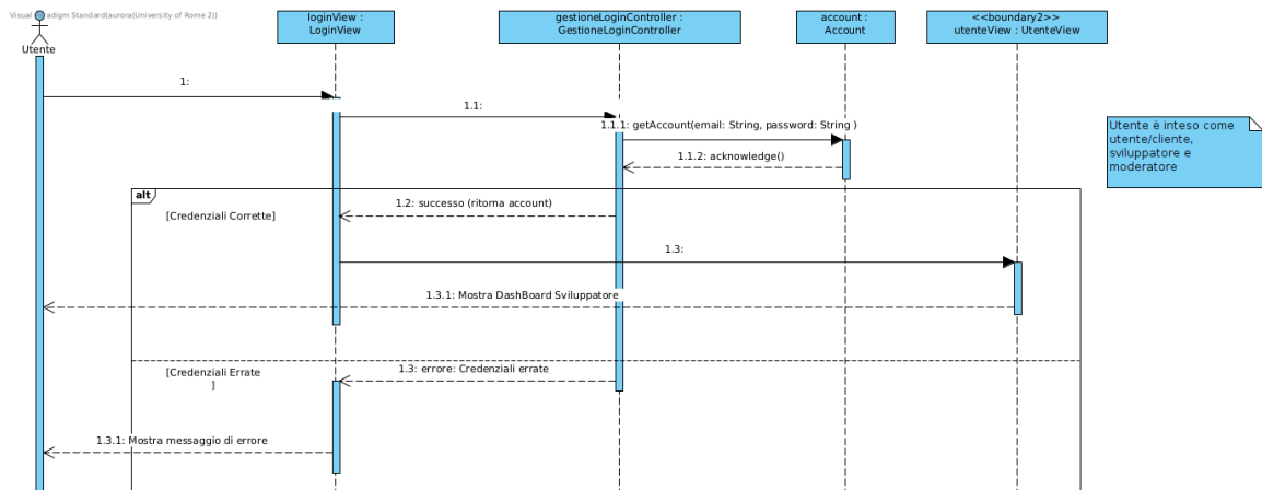
Figura 23: Sequence Diagram - Login
